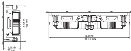
MOUNTING DEPTH/ MINIMUM CUTOUT
