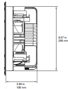
MOUNTING DEPTH/ MINIMUM CUTOUT
