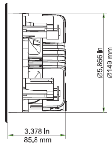
MOUNTING DEPTH/ MINIMUM CUTOUT
